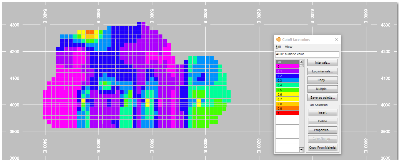
Figure 14-10: Long-section View of Shaft Vein Block Model looking North (grid lines=200')
