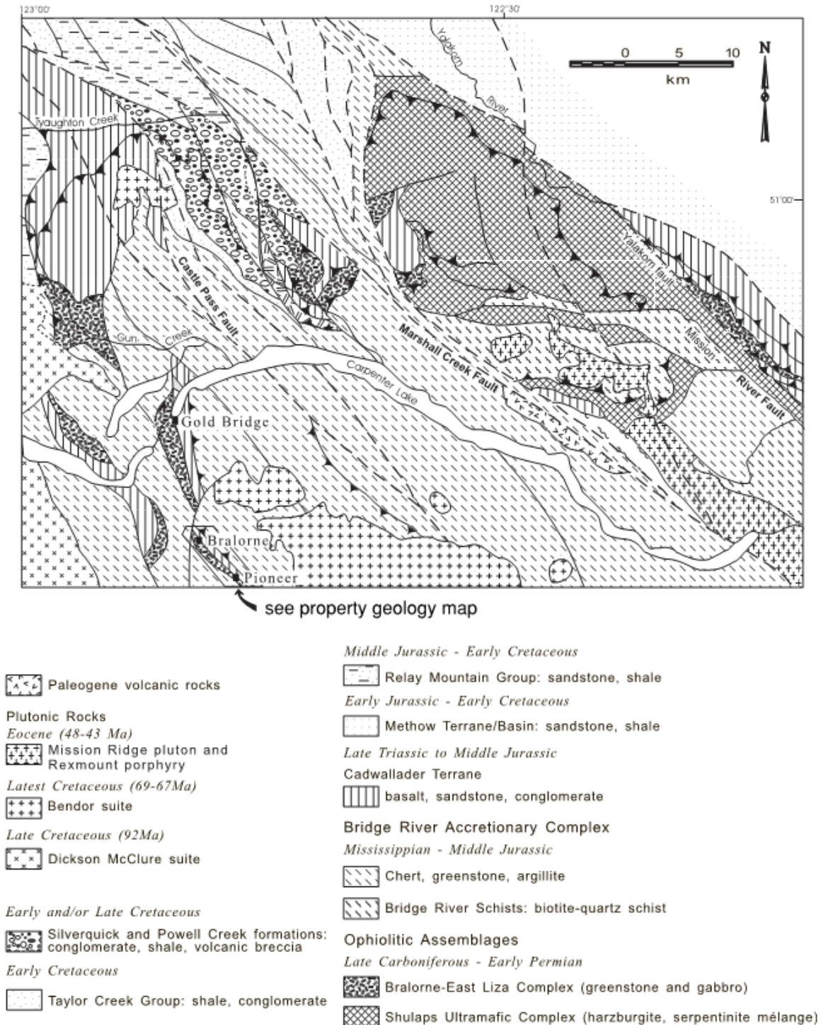
Figure 7-3: Local Geological Setting of the Bralorne Property
